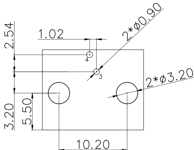
RECOMMENDED PCB LAYOUT TOP VIEW (TOL: \pm 0.05 )
