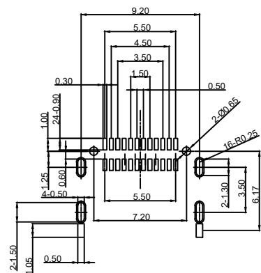
RECOMMEND P.C.B LAYOUT (COMPONENT SIDE)
