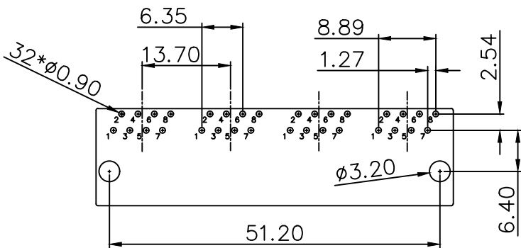
RECOMMENDED PCB LAYOUT TOP VIEW(TOL:±0.05)
