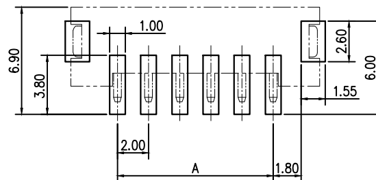
PCB LAYOUT
