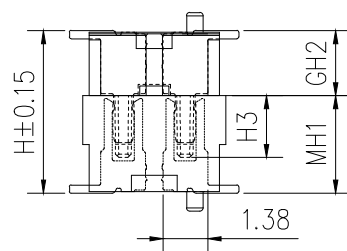
ASSEMBLY
