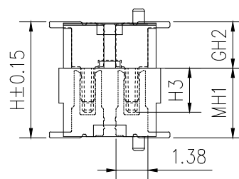
ASSEMBLY
