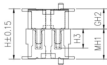
ASSEMBLY
