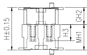
ASSEMBLY
