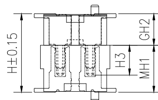
ASSEMBLY
