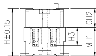
ASSEMBLY
