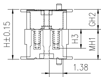
ASSEMBLY
