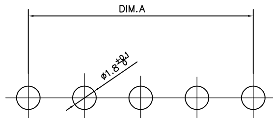
PCB LAYOUT
